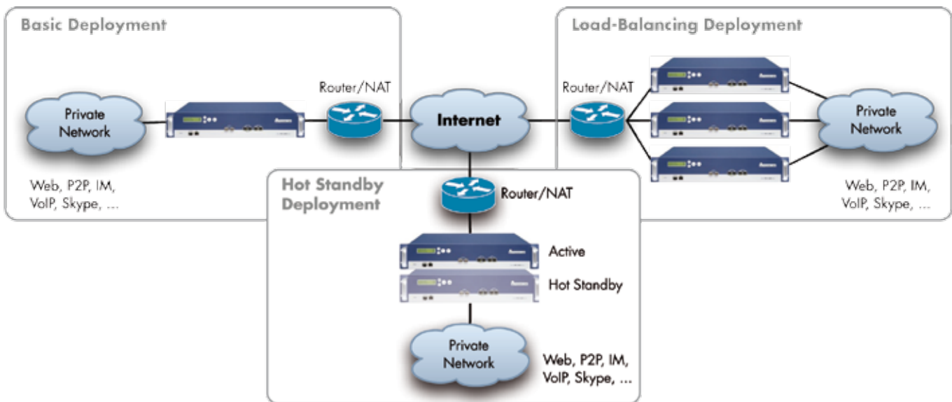
PRX Traffic Manager – Deployment Scenarios
